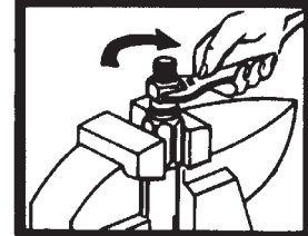
7. Screw nipple into socket, using wrench on hex of nipple. After assembled, blow out with air pressure to remove any loose particles and inspect.
