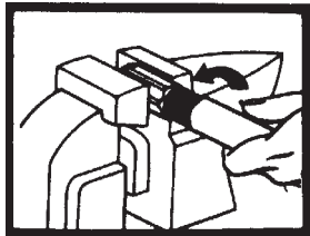
4. Place socket in vise and screw hose in counter-clockwise, using body weight against hose to start threading. Tighten until hose bottoms, then back off 1/4 turn.
